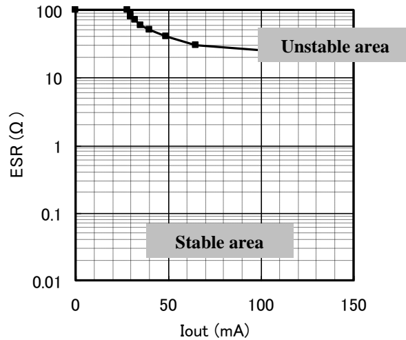
Figure 2. Stability area graph Condition: Vin=Vout(typ)-1.5V Cin=0.1μF, Cout=1.0μF (MLCC)
