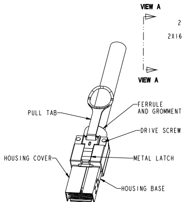
P1 ISOMETRIC VIEW SCALE 2:1
