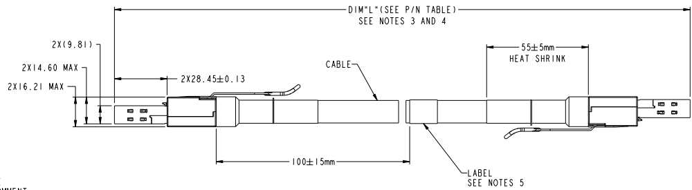
END P1 CABLE CONNECTOR CXP (PASSIVE) PLUG
