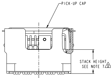
SECTION D-D SCALE 5:1
