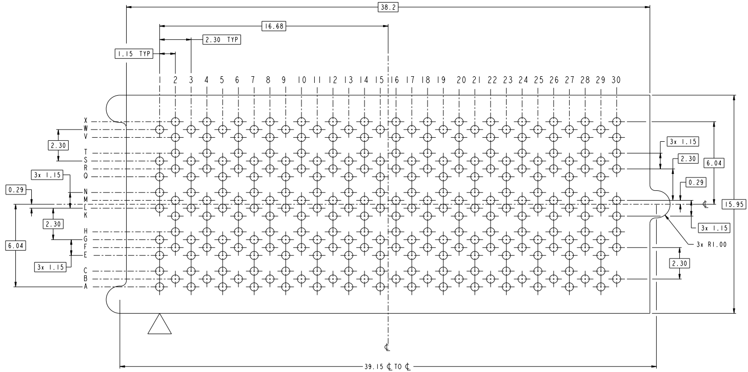
BOARD LAYOUT 15 IMLA CONNECTOR SEE NOTE 4 SCALE 10:1
