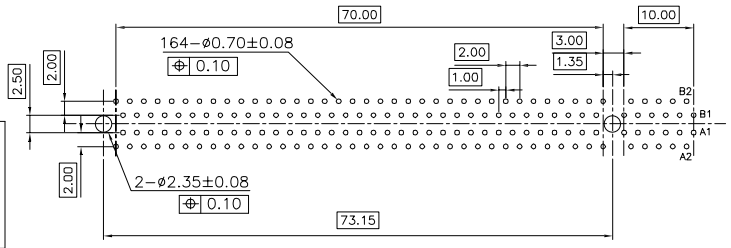
RECOMMENDED FOOTPRINT LAYOUT
