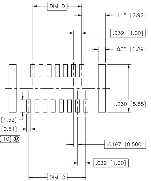
RECOMMENDED STENCIL LAYOUT FOR RECEPTACLE
