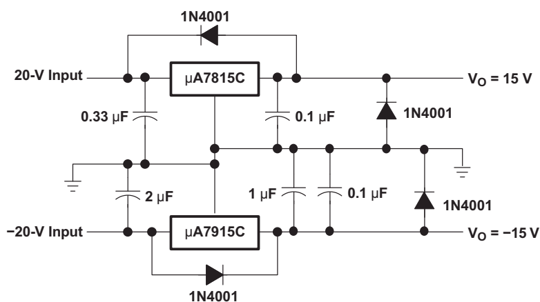
Figure 9. Regulated Dual Supply
