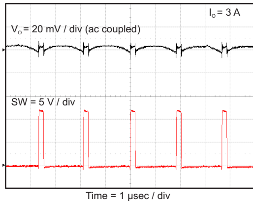
Figure 37. TPS563219 Output Voltage Ripple
