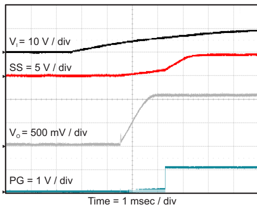
Figure 39. TPS563219 Start Up Relative To V i
