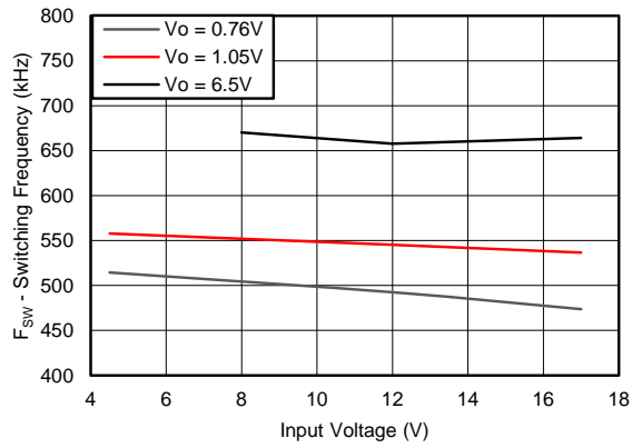
Figure 7. Switching Frequency vs Input Voltage
