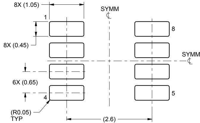
LAND PATTERN EXAMPLE SCALE:15X
