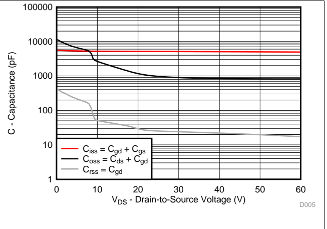
Figure 5. Capacitance
