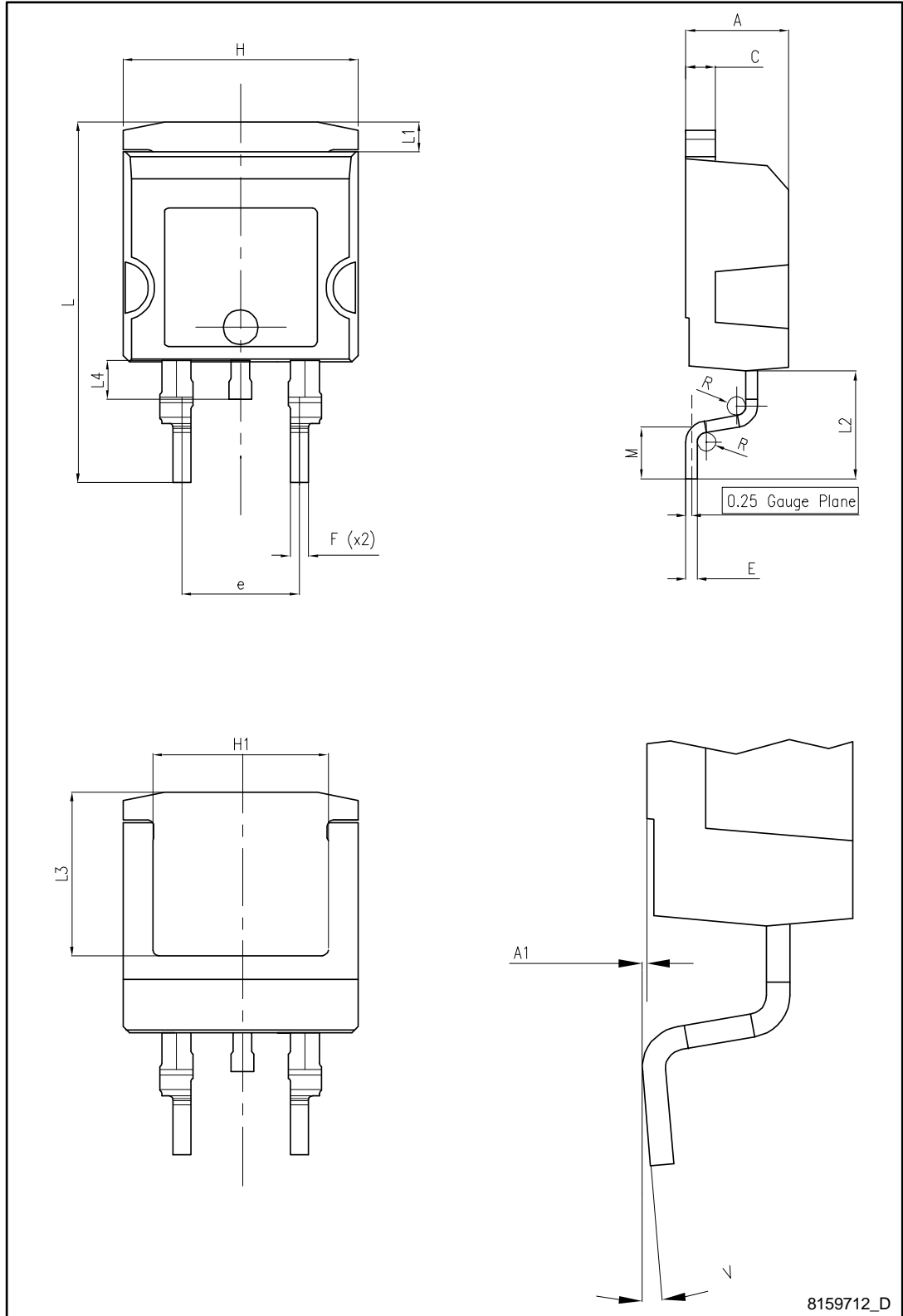
Figure 23: H 2 PAK-2 package outline
