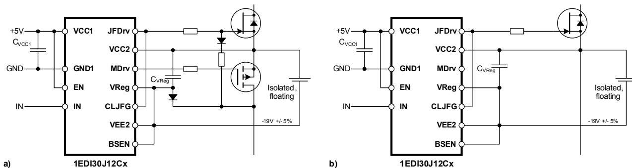
Figure 11 Isolated and floating direct supply, a) cascode configuration, b) only JFET
