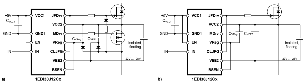
Figure 10 Isolated and floating supply, a) cascode configuration, b) only JFET
