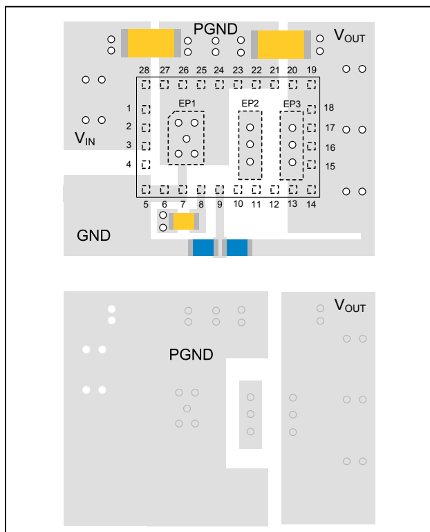
Figure 2. Layout Recommendation
