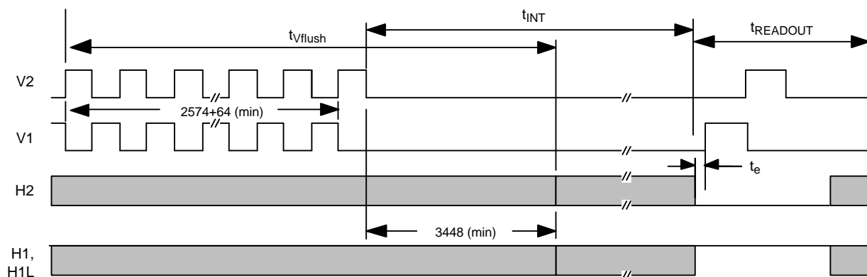
Figure 19. Power-Up Flush Cycle
