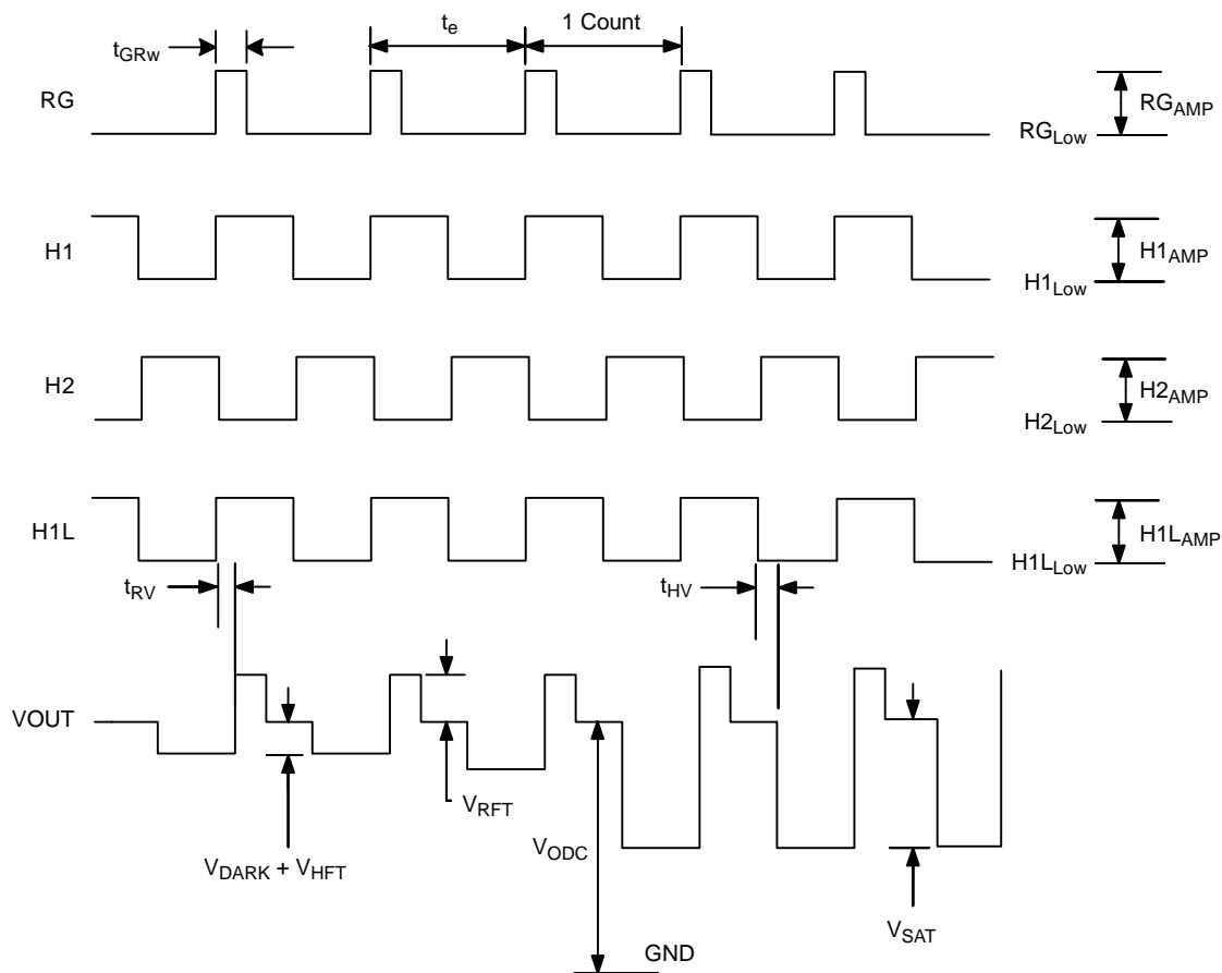
Figure 17. Pixel Timing
