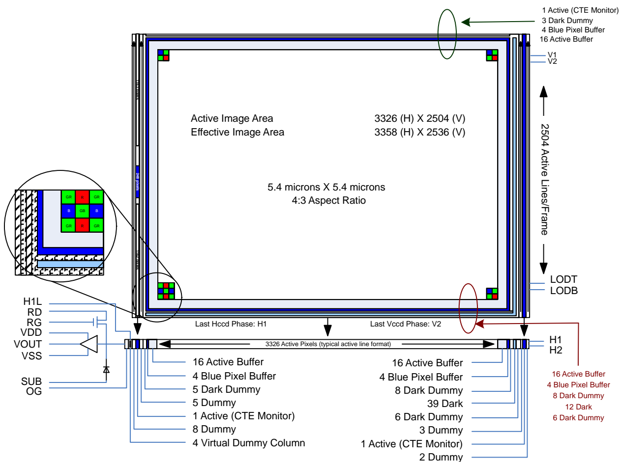
Figure 2. Block Diagram (Color)
