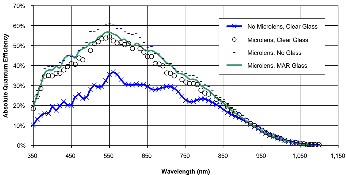
Figure 8. Typical Quantum Efficiency (All Monochrome Versions)
