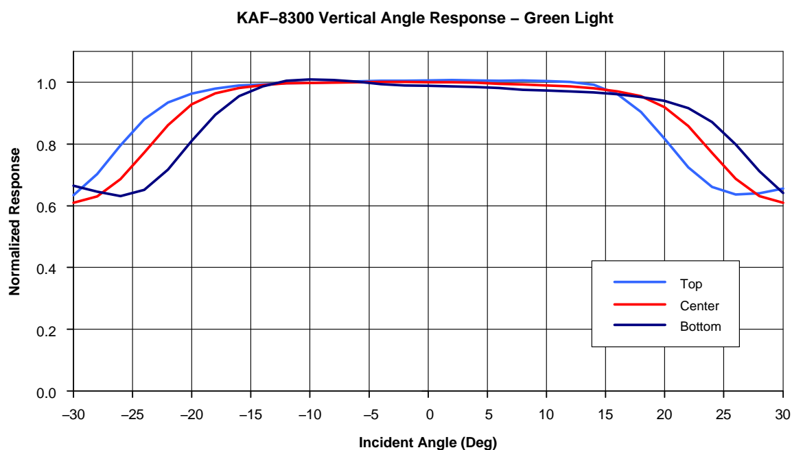
Figure 10. Typical Angular Response (Monochrome with Microlens)
