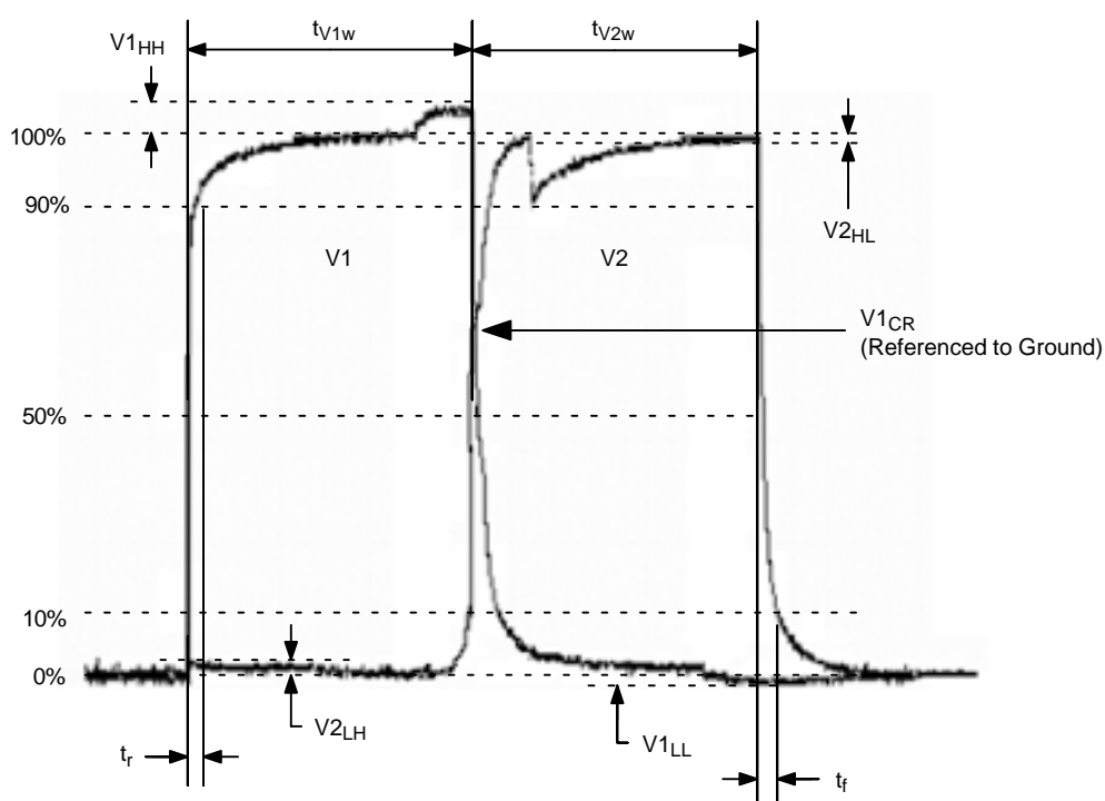
Figure 15. Frame Timing Edge Alignment
