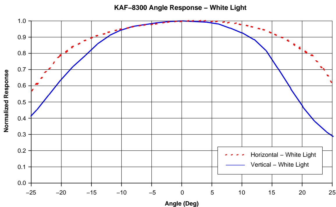
Figure 9. Typical Angular Response (Color Version)
