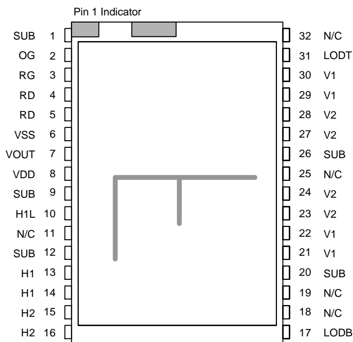
Figure 6. Pinout Diagram
