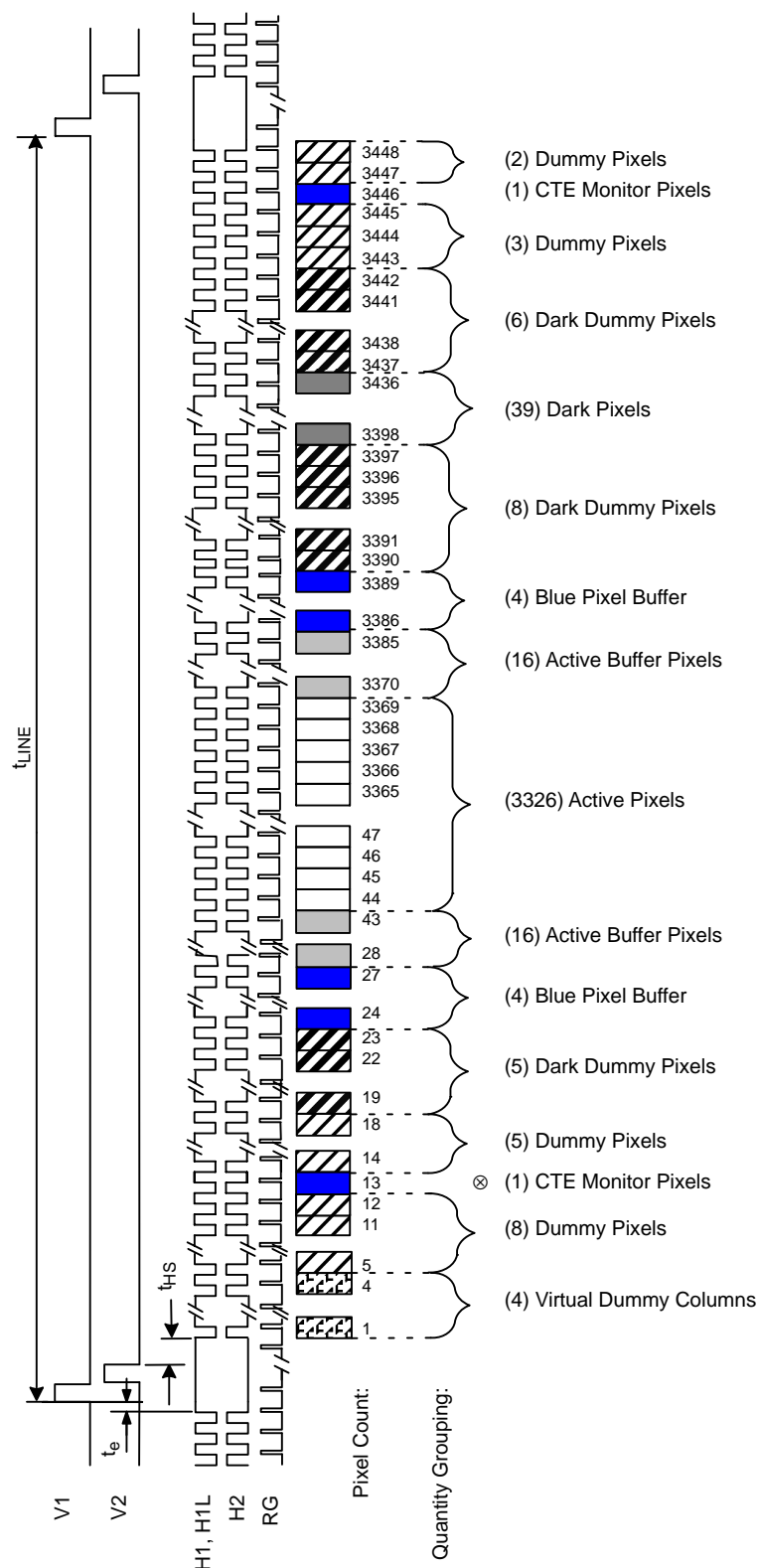
Figure 16. Line Timing
