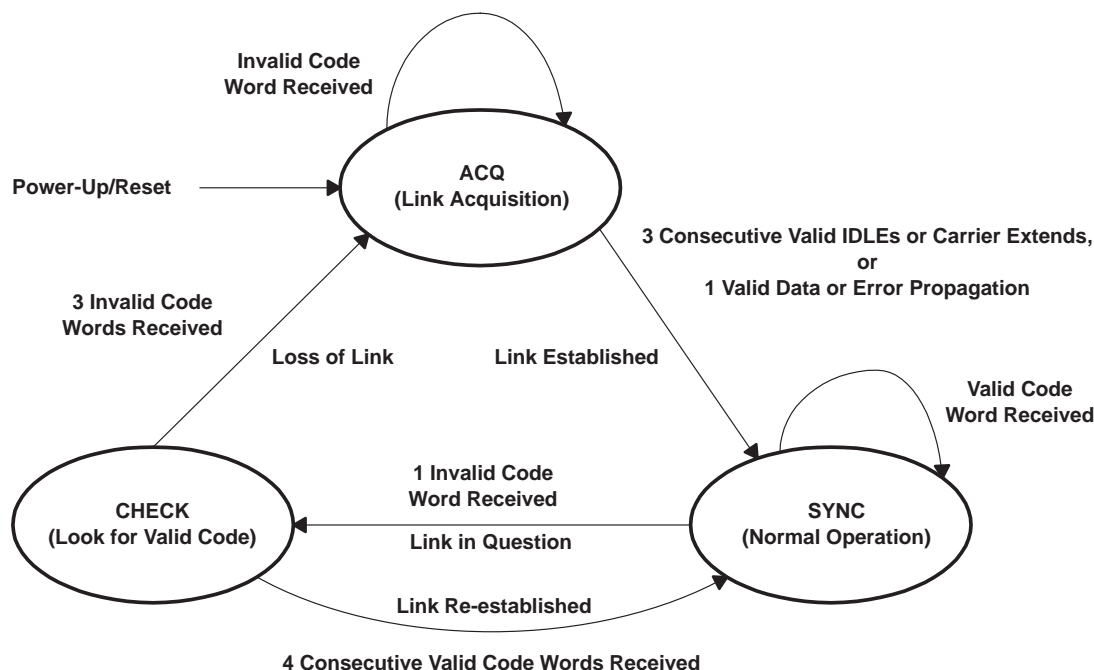
Figure 5. Initialization and Synchronization State Diagram
