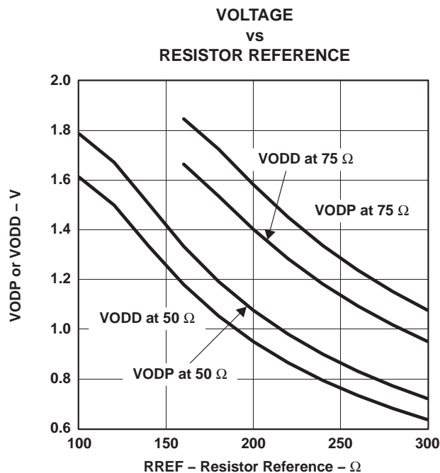
Figure 13. Differential Transmitter Voltage
