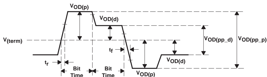
Figure 11. Differential- and Common-Mode Output Voltage Definitions
