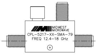
BACKSIDE MARKING
