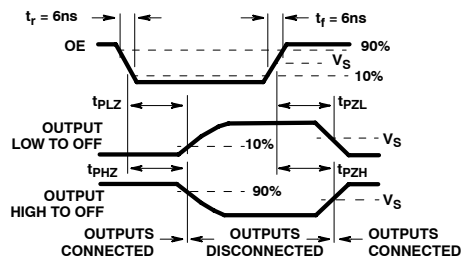
FIGURE 3. ENABLE AND DISABLE TIMES
