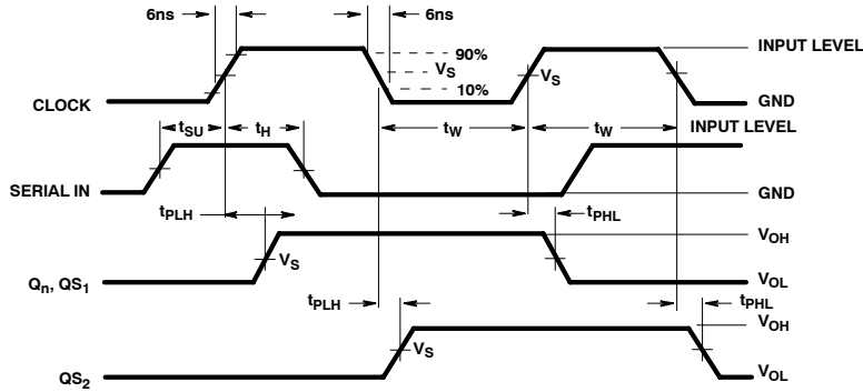
FIGURE 1. DATA PROPAGATION DELAYS, SET-UP AND HOLD TIMES
