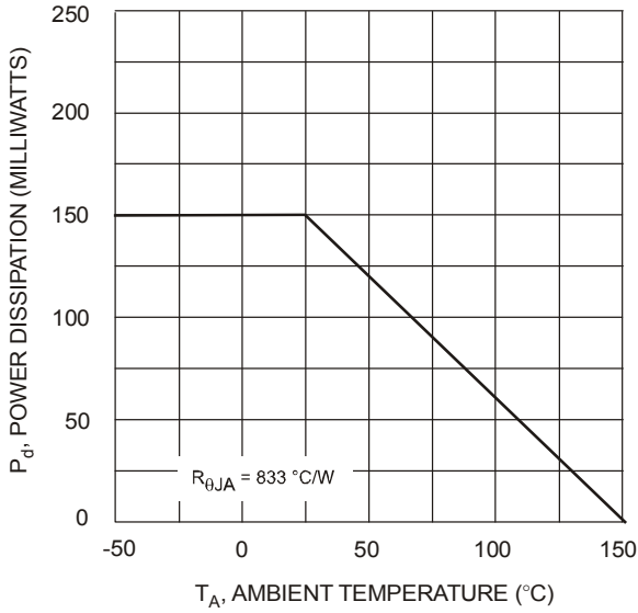
Fig. 1 Derating Curve
