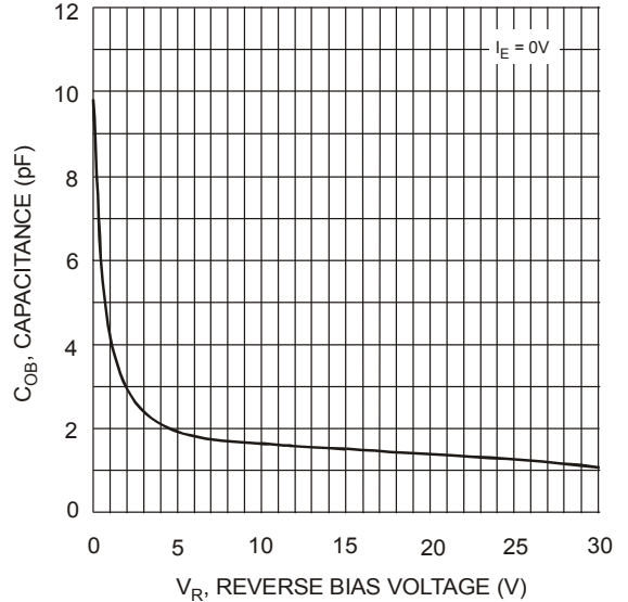
Fig. 4 Output Capacitance
