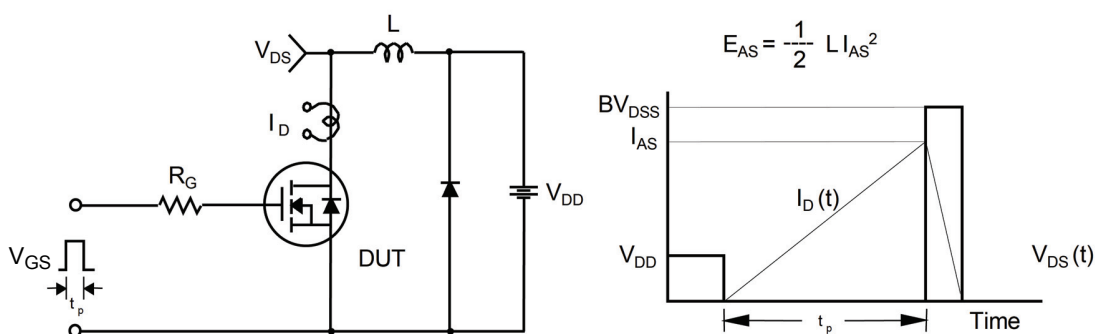
Figure 15. Unclamped Inductive Switching Test Circuit & Waveforms
