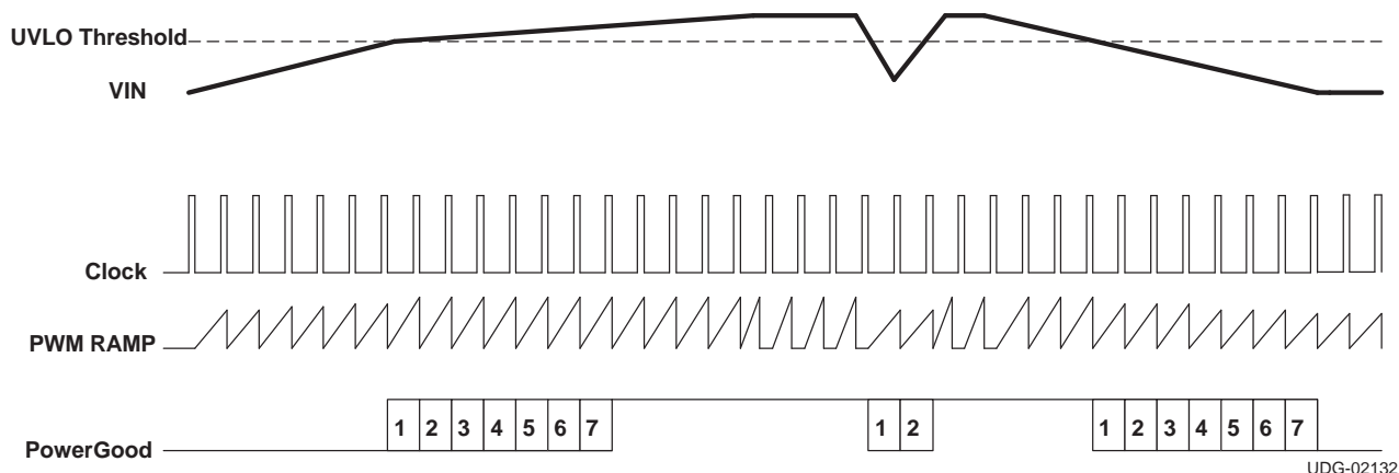
Figure 4. Undervoltage Lockout Operation
