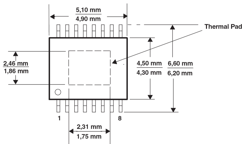
Figure 13. PowerPAD Dimensions
