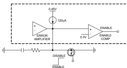
Figure 1. Chip Enable Function
