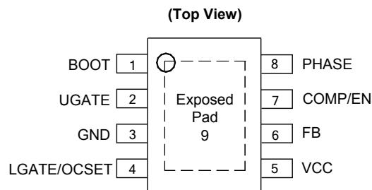
(SO-8EP/ MP Package)
