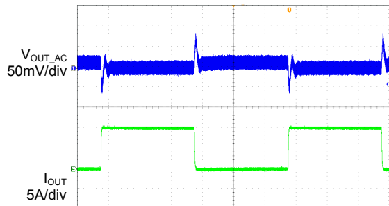
Load Transient Response ( V_{IN} = 12V , V_{OUT} = 1.5V , I_{OUT} = 0A to 10A )
