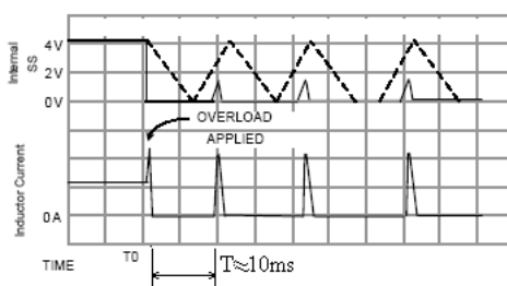
Figure 4. Hiccupped Over Current Protection
