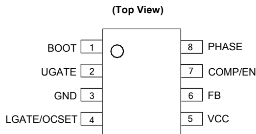
(SO-8/ M Package)
