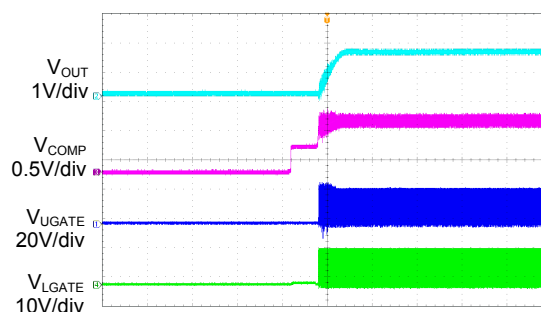
Enable-on Waveform ( V_{IN} = 12V , V_{OUT} = 1.5V , I_{OUT} = 0A )
