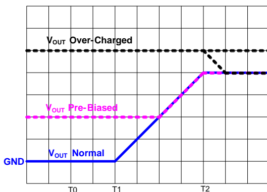
Figure 2. Start-up Behavior with Pre-biased Output Voltage
