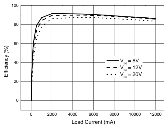
Efficiency vs. Load Current @ V_{OUT} = 2.5V
