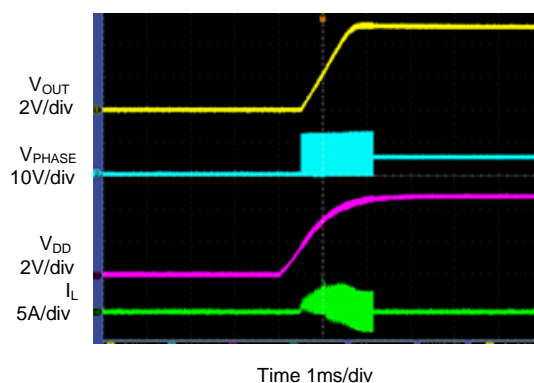
Power ON from VDD @DEM
