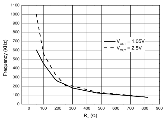
Frequency vs. R_T
