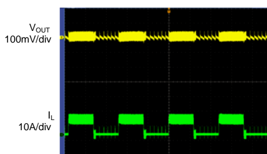
Load Transient Response @ DEM
