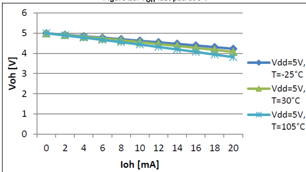
Figure 28. V_{OH} fast pad at 5 V
