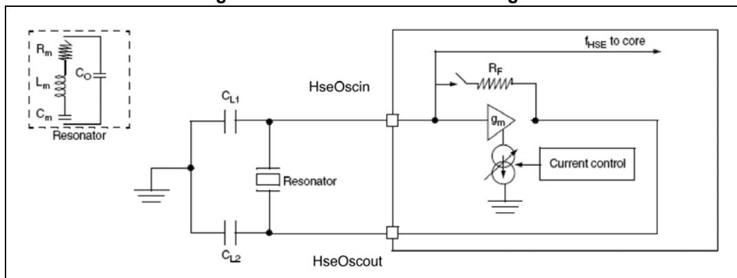
Figure 21. HSE oscillator circuit diagram
