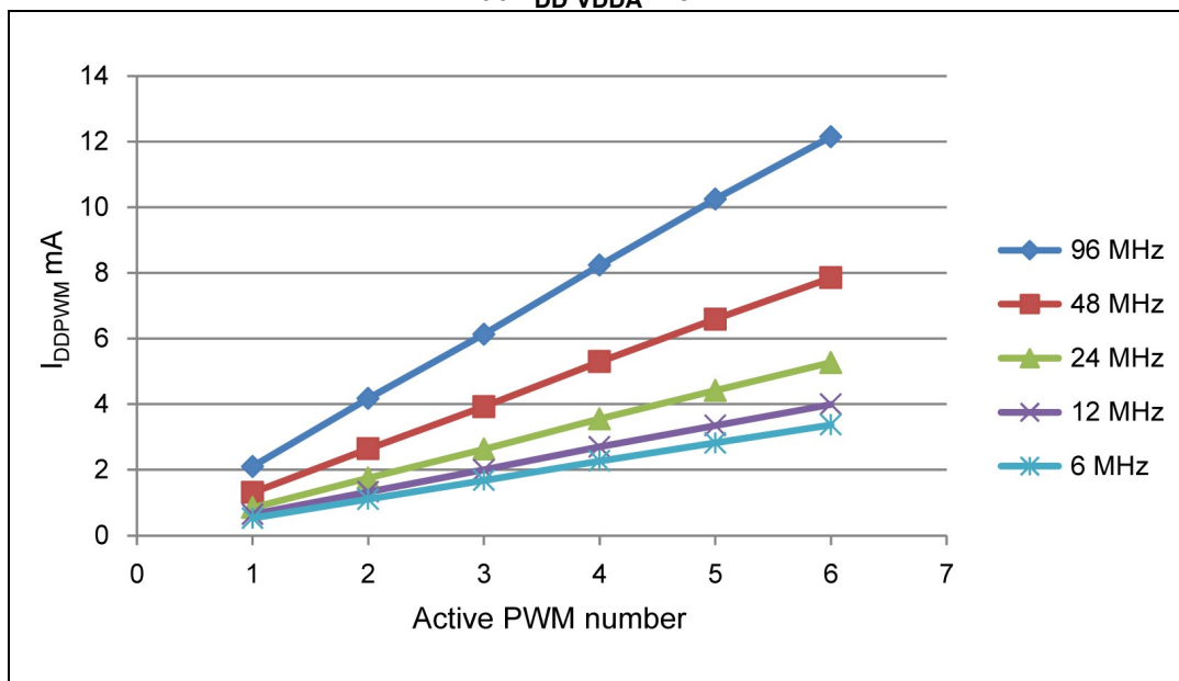
Figure 16. PWM current consumption with f_{\text{SMED}} = \text{PLL } f_{\text{PWM}} = 0.5\text{ MHz} at V_{\text{DD}}/V_{\text{DDA}} = 5\text{ V}
