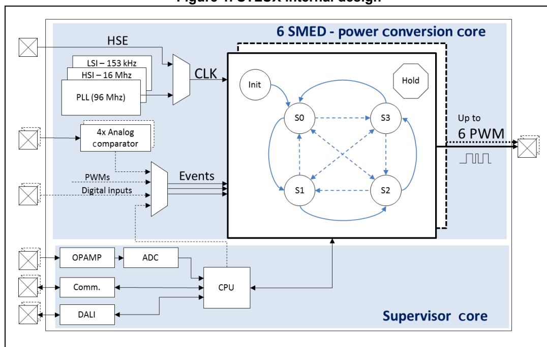
Figure 1. STLUX internal design
