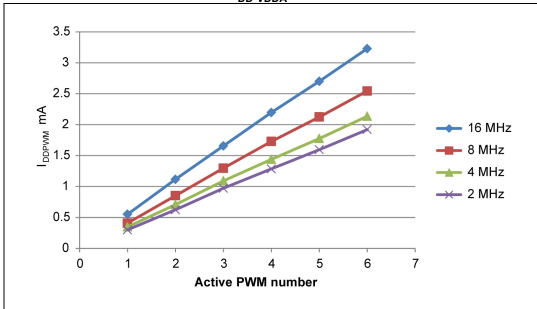
Figure 18. PWM current consumption with f_{SMED} = HSI f_{PWM} = 0.5 MHz at V_{DD}/V_{DDA} = 3.3 V
