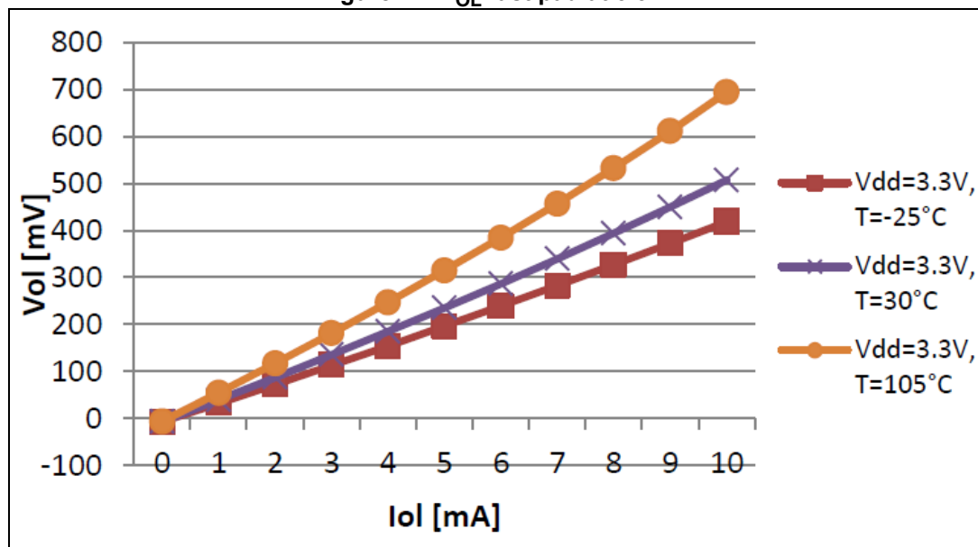
Figure 27. V_{OL} fast pad at 3.3 V
