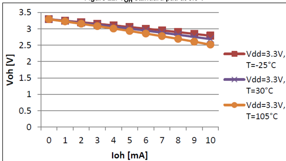
Figure 22. V_{OH} standard pad at 3.3 V
