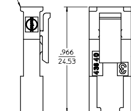
MATED MICRO-FIT CONNECTOR
