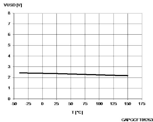
Figure 24: Undervoltage shutdown
