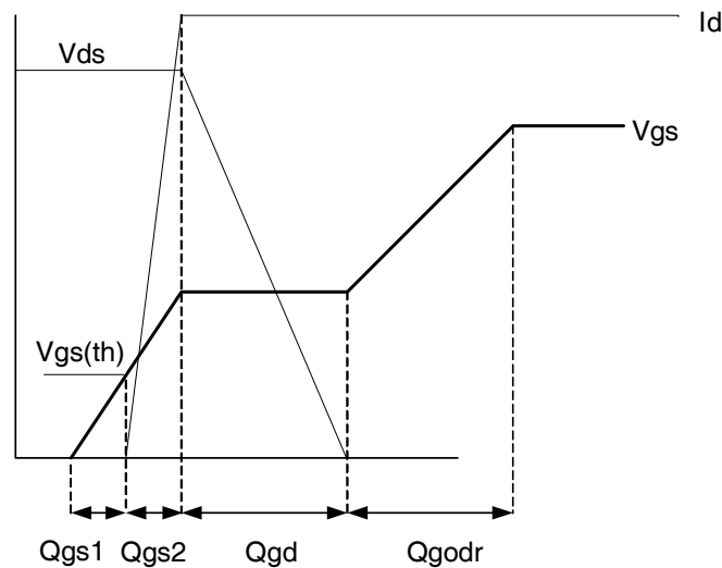
Fig 19. Gate Charge Waveform
