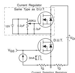
Fig 15. Gate Charge Test Circuit
