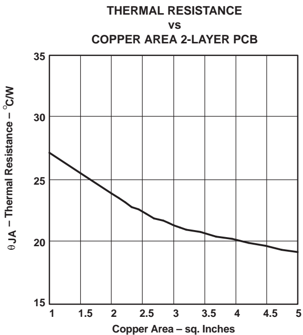
Figure 47. Thermal Resistance
