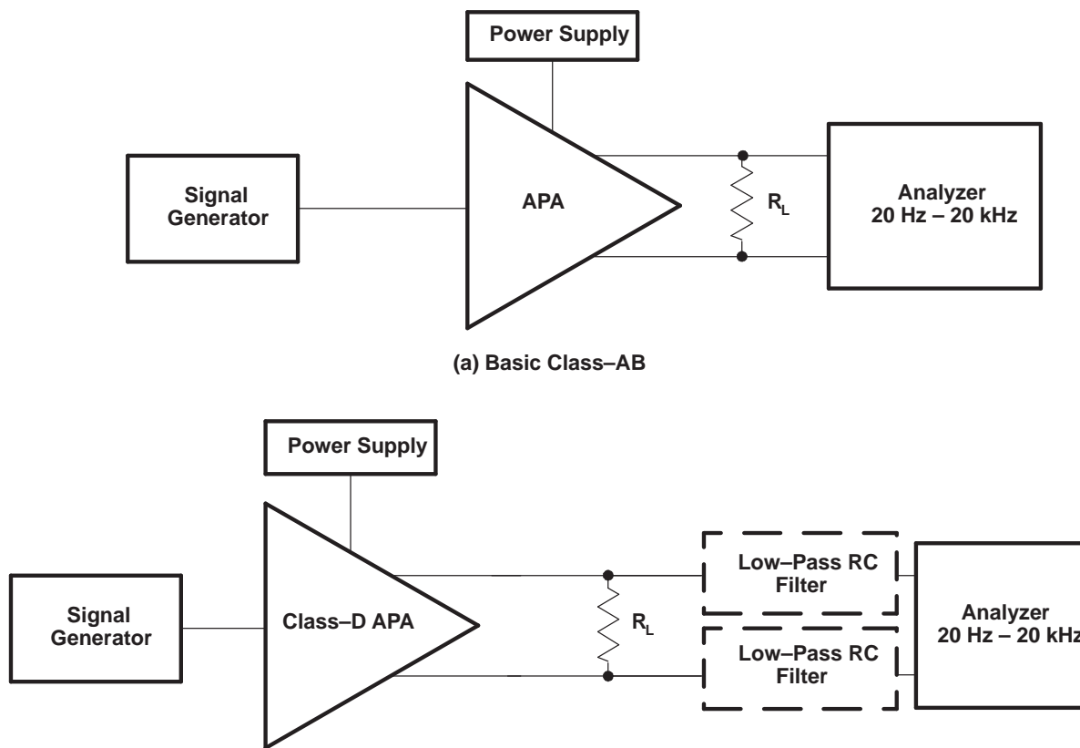
(b) Filter-Free and Traditional Class-D
