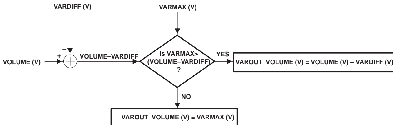
Figure 42. Block Diagram of VAROUT Volume Control
