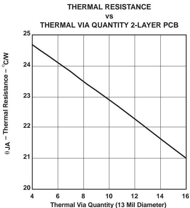
Figure 48. Thermal Resistance
