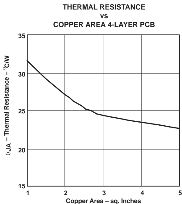
Figure 47. Thermal Resistance
