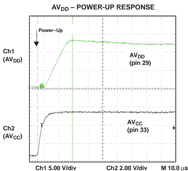
Figure 46. Power-Up Response
