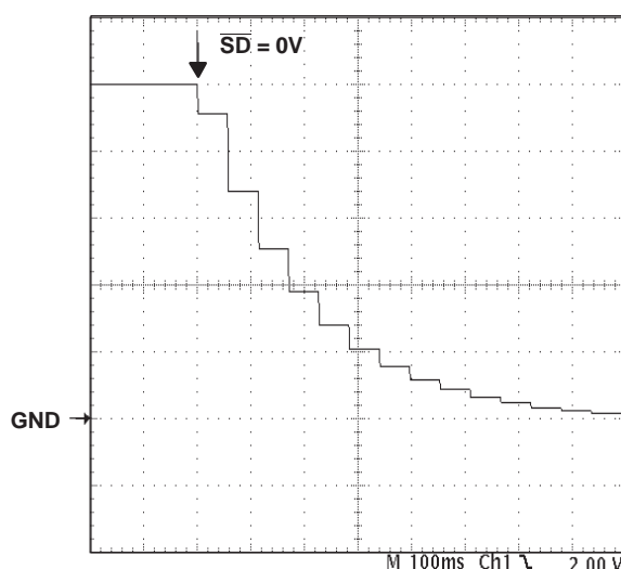
Figure 44. Differential Output With \overline{\text{FADE}} (Terminal 30) Held Low
