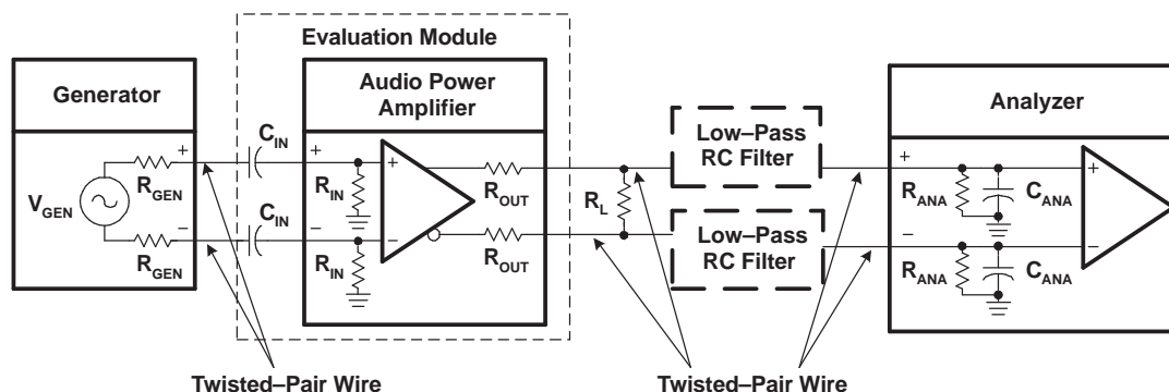
Figure 50. Differential Input—BTL output Measurement Circuit
