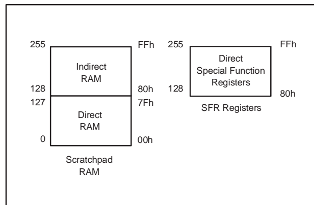
Figure 22. Register Map
