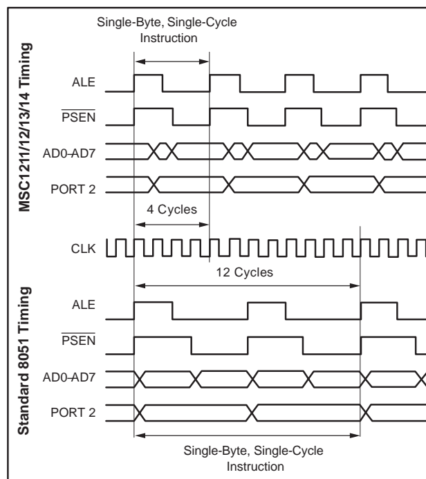
Figure 10. Comparison of MSC1211/12/13/14 Timing to Standard 8051 Timing
