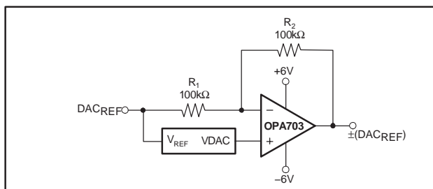
Figure 18. Bipolar Operation with the DAC
