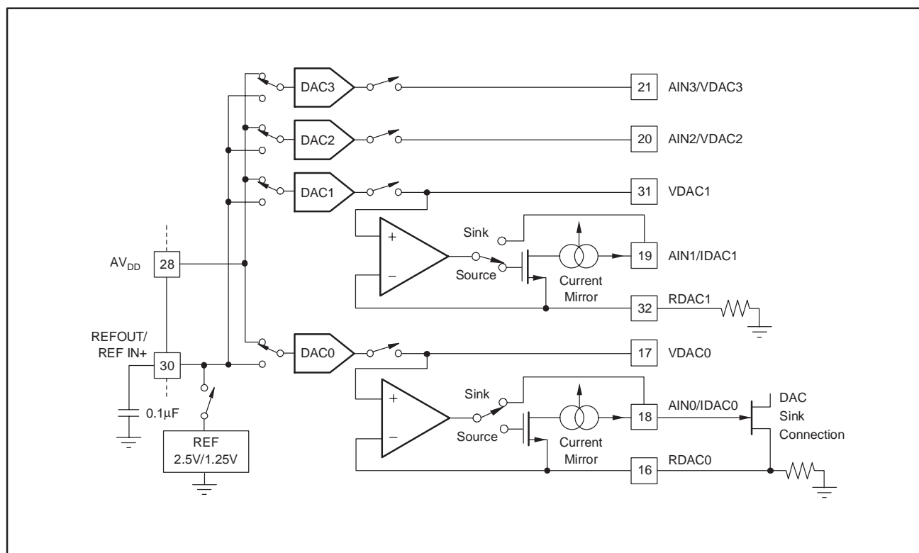
Figure 17. DAC Architecture
