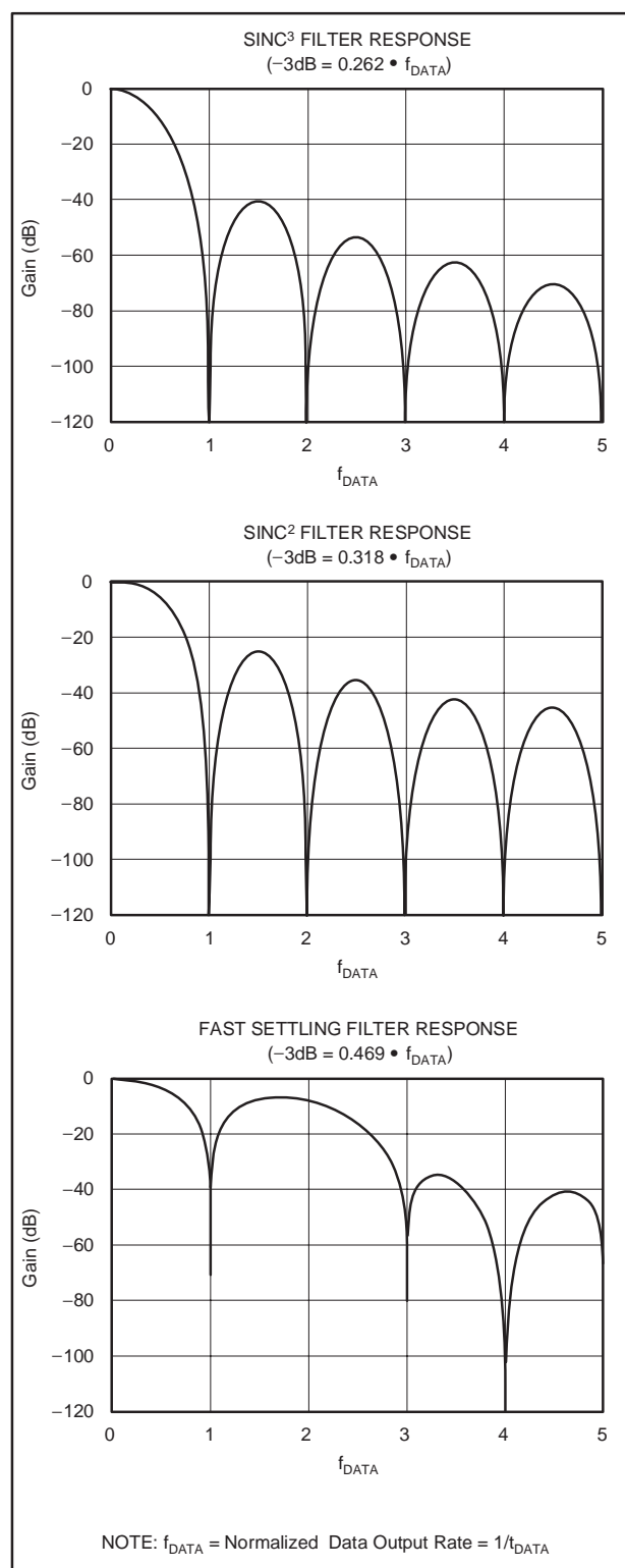
Figure 16. Filter Frequency Responses
