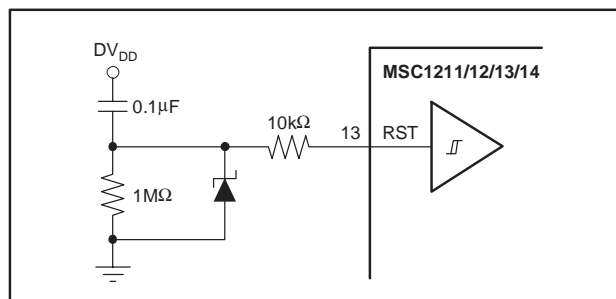
Figure 19. Typical Reset Circuit
