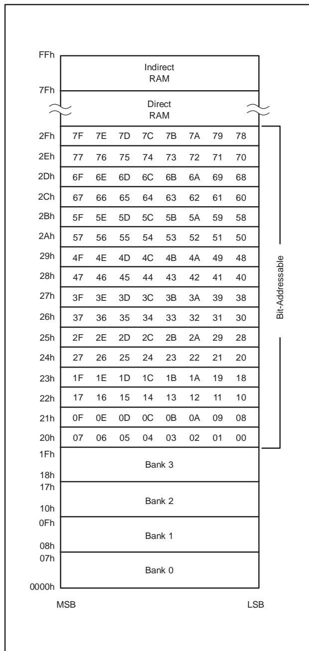
Figure 23. Scratchpad Register Addressing
