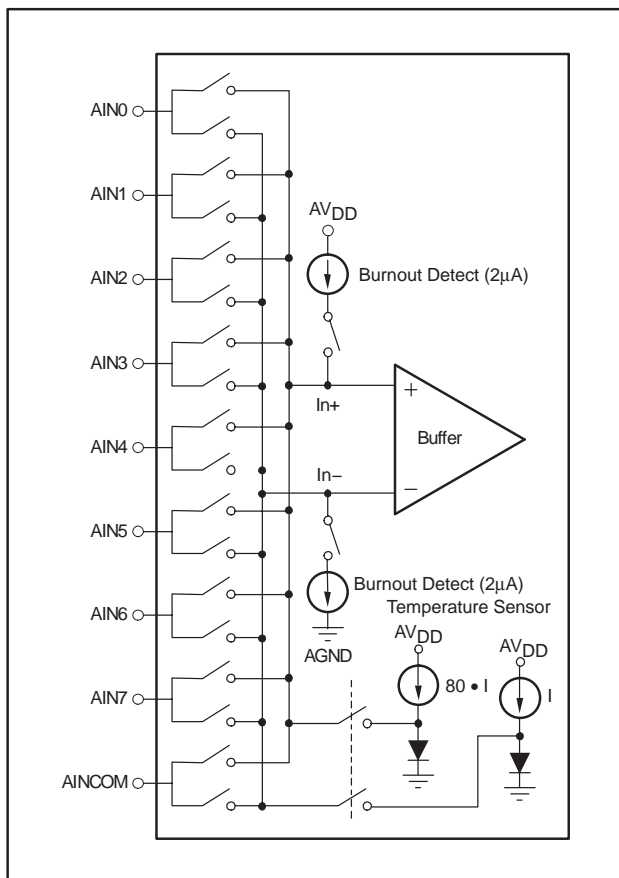
Figure 13. Input Multiplexer Configuration
