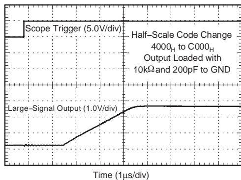
VDAC HALF-SCALE SETTLING TIME
