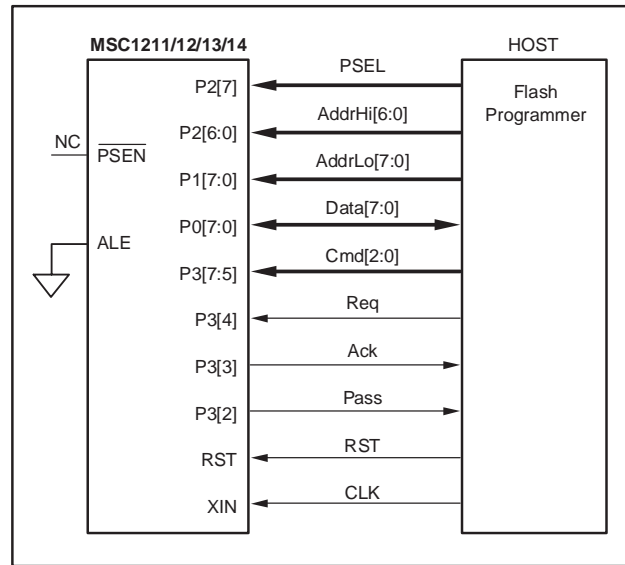
Figure 24. Parallel Programming Configuration
