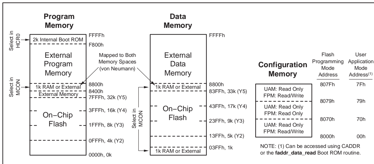
Figure 20. Memory Map
