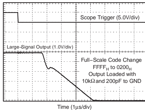
VDAC FULL-SCALE SETTLING TIME
