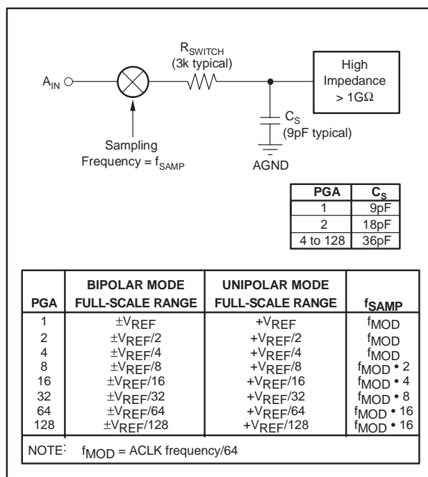
Figure 14. Analog Input Structure
