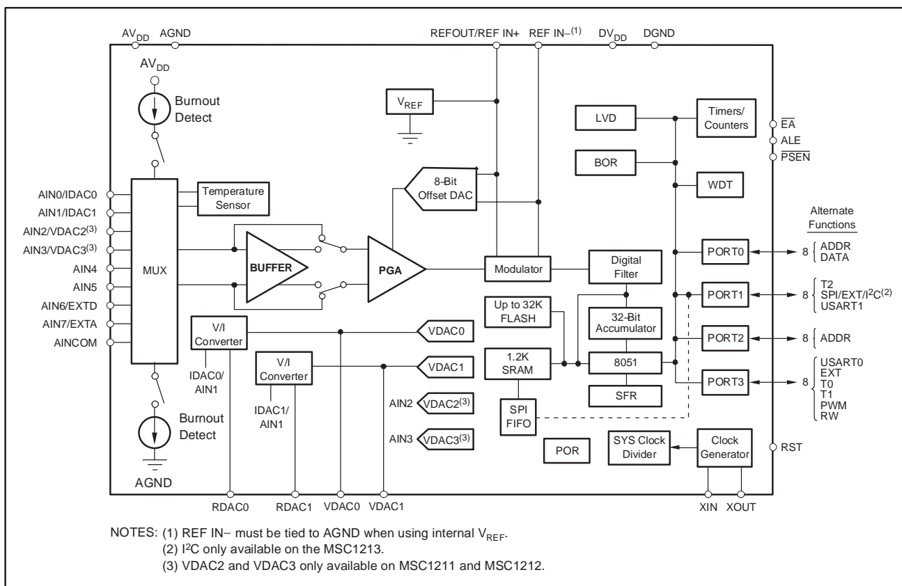
Figure 8. Block Diagram
