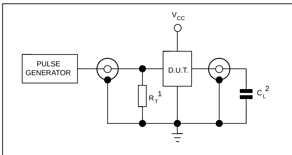
Figure 4: Test circuit
