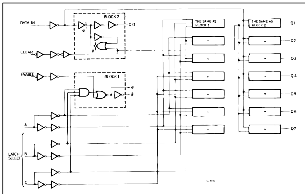
Figure 3: Logic diagram
