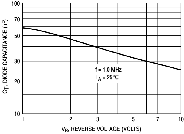
Figure 1. Diode Capacitance
