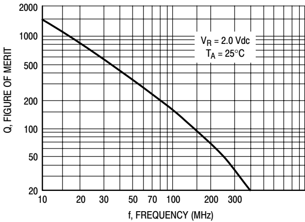
Figure 3. Figure of Merit versus Frequency
