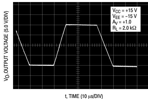
Figure 7. Large Signal Transient Response
