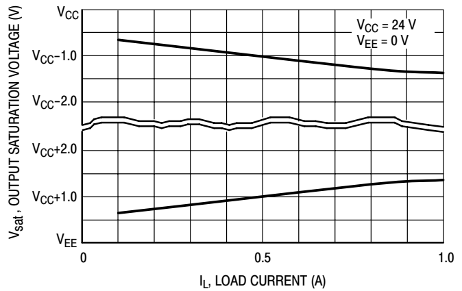
Figure 3. Output Saturation Voltage versus Load Current
