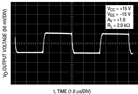
Figure 6. Small Signal Transient Response
