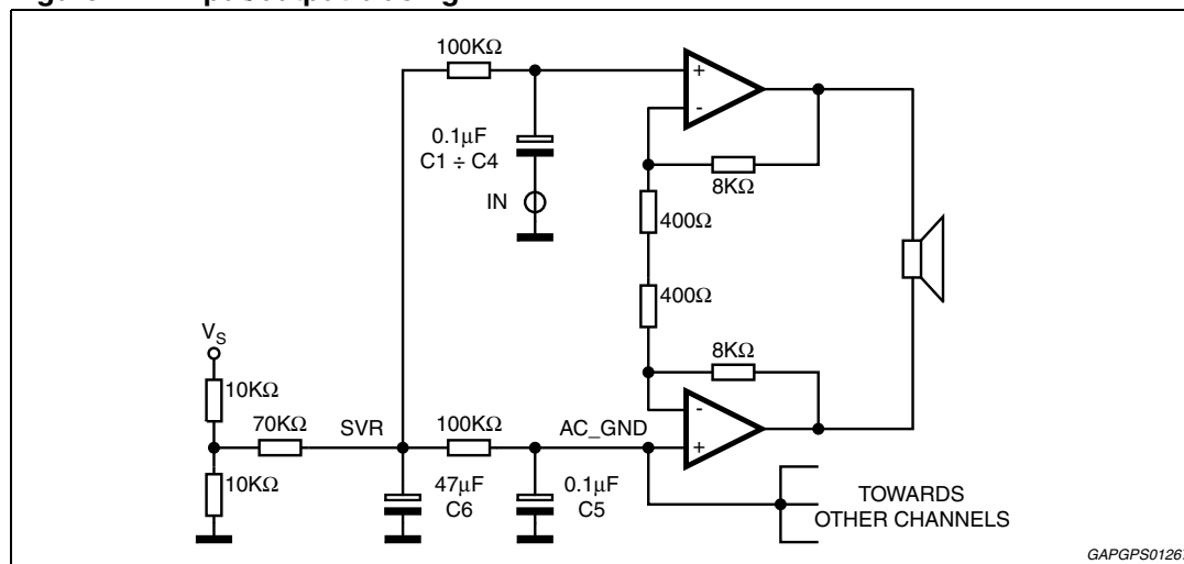
Figure 14. Input/output biasing
