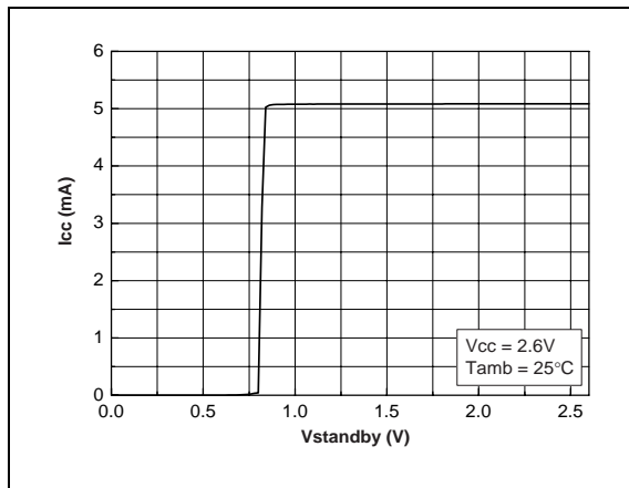
Fig. 51 : Current Consumption vs Standby Voltage @ Vcc = 2.6V
