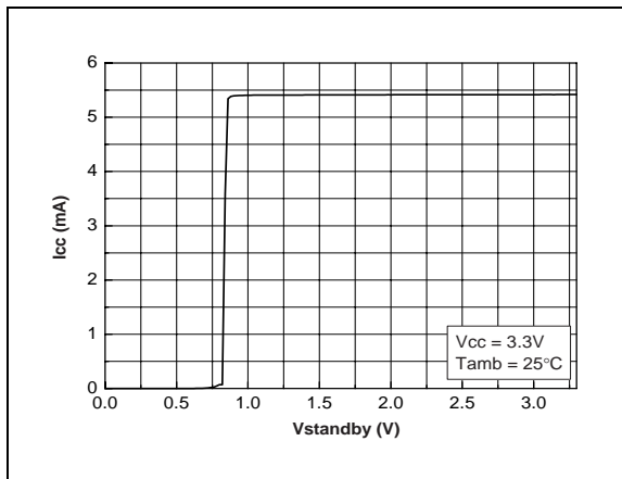
Fig. 50 : Current Consumption vs Standby Voltage @ Vcc = 3.3V
