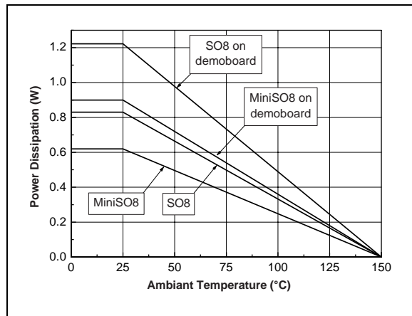
Fig. 20 : Power Derating Curves
