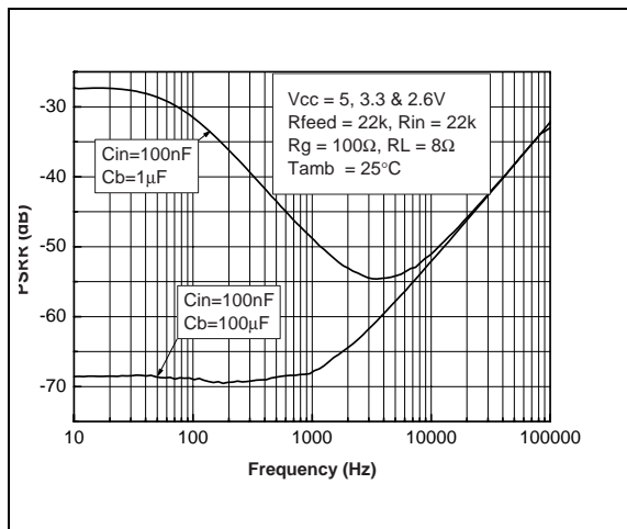
Fig. A : PSRR changes with C b
