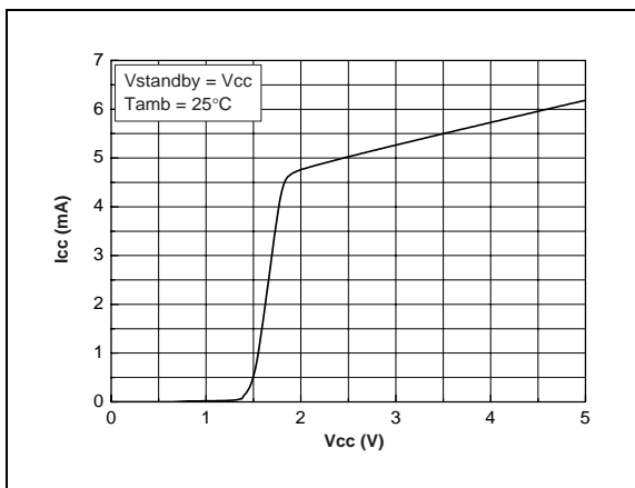
Fig. 48 : Current Consumption vs Power Supply Voltage
