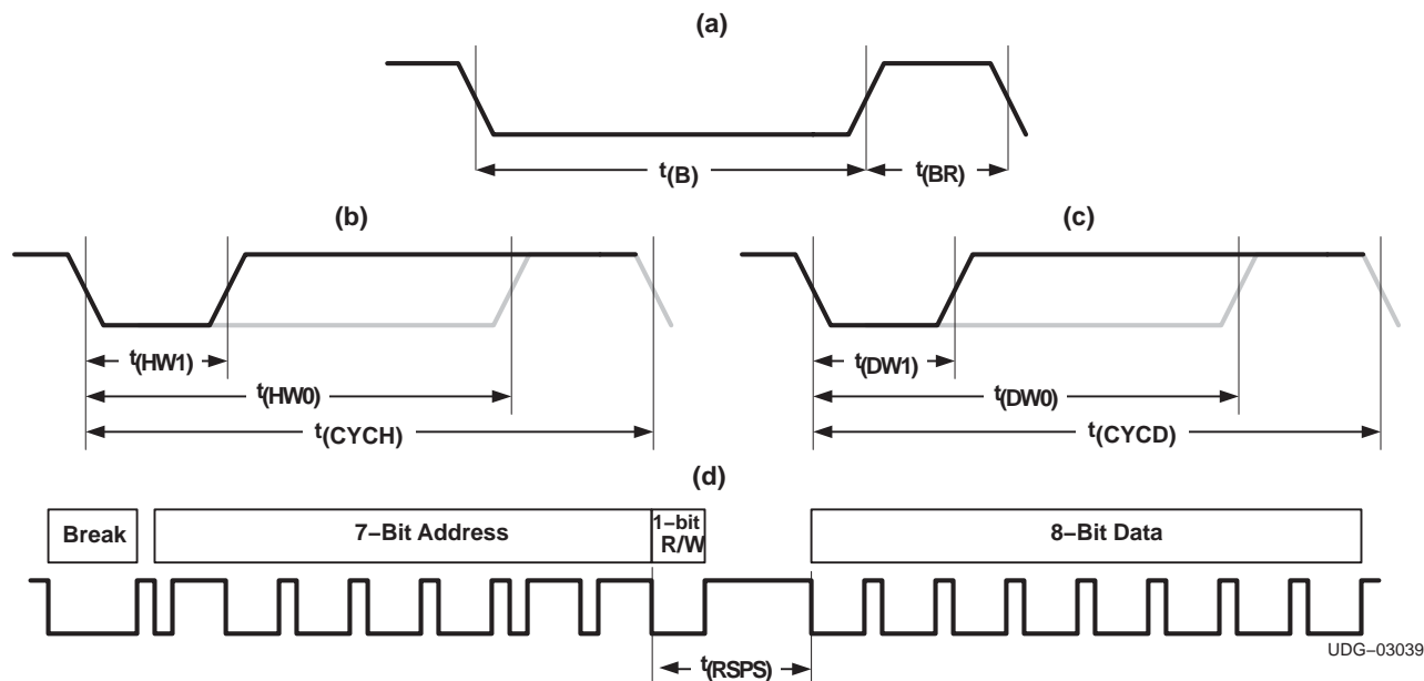
Figure 1. HDQ Bit Timing Diagrams
