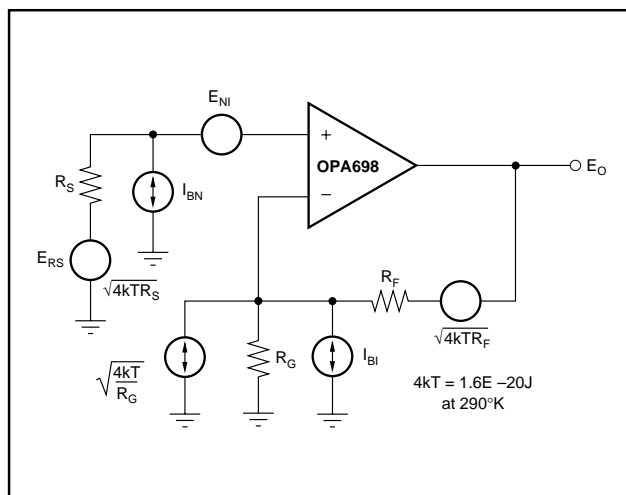
FIGURE 24. Op Amp Noise Analysis Model.
