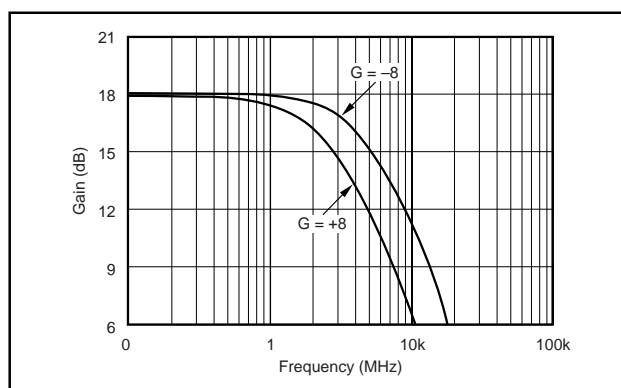
FIGURE 4. G = +8 and -8 Frequency Response.
