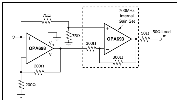
FIGURE 11. High-Speed Full Wave Rectifier #2.
