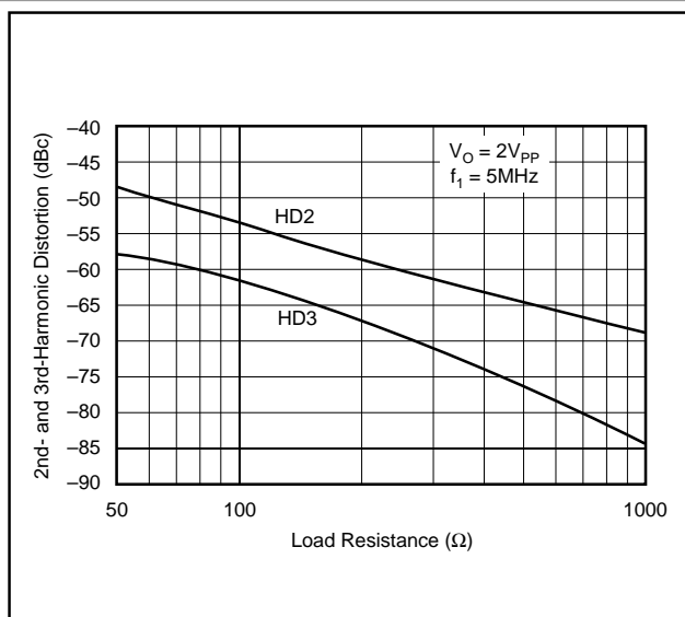
FIGURE 23. 5MHz Harmonic Distortion vs Load Resistance.
