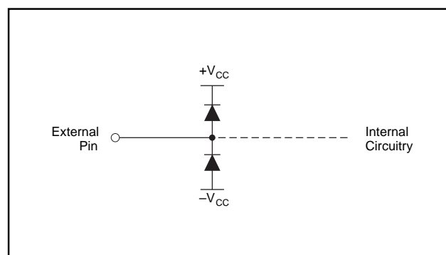
FIGURE 26. Internal ESD Protection.
