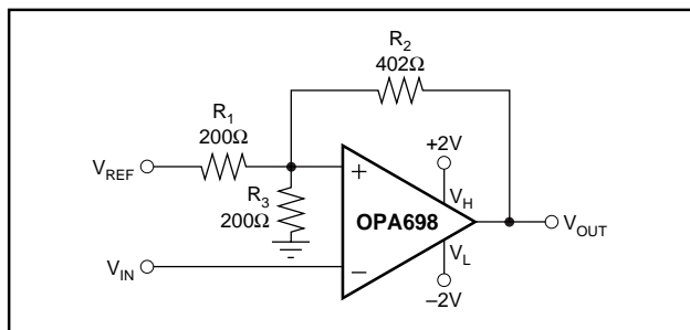
FIGURE 15. Very High-Speed Schmitt Trigger.
