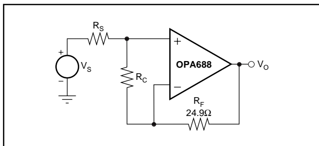
FIGURE 17. Unity-Gain Buffer.
