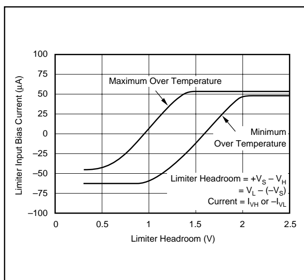
FIGURE 20. Limiter Bias Current vs Bias Voltage.
