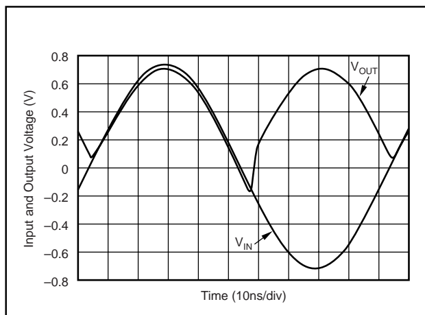
FIGURE 12. 10MHz Sinewave Rectified.
