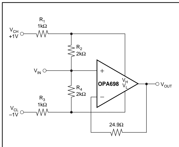
FIGURE 13. Soft-Clipping Circuit.
