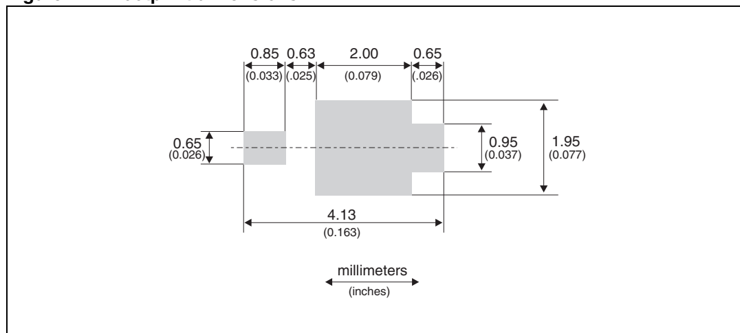
Figure 21. Footprint dimensions
