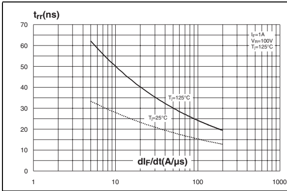
Figure 9. Reverse recovery time versus dl_F/dt (90% confidence)
