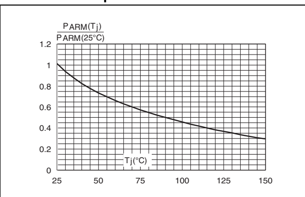
Figure 5. Normalized avalanche power derating junction temperature
