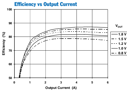
PTH12000L Characteristic Data, V_{in} = 12\text{ V} (See Note A)
