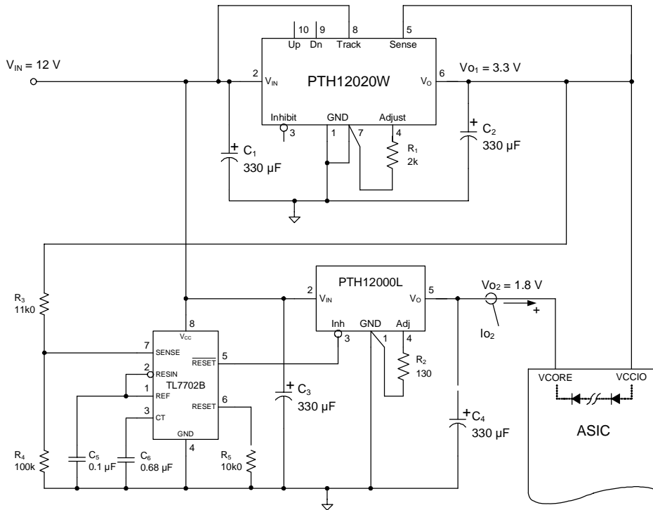
Figure 3-4; Application Circuit Demonstrating Pre-Bias Startup
