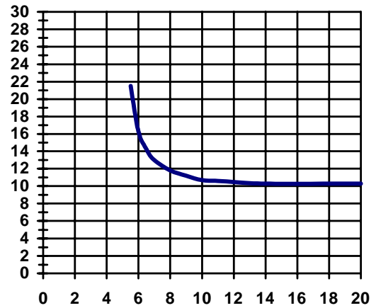
Figure 10 - Rds(on) (mΩ) vs Vcc (V)
