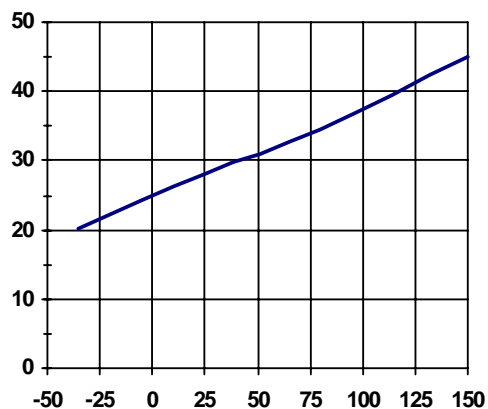
Figure 6 - IN1 (2) current (µA) vs Tj (°C)
