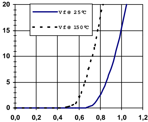
Figure 9 - Body diode : Ids (A) vs Vds (V)
