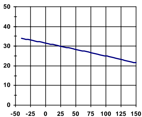
Figure 8 - Typ. I shutdown (A) vs Tj (°C)
