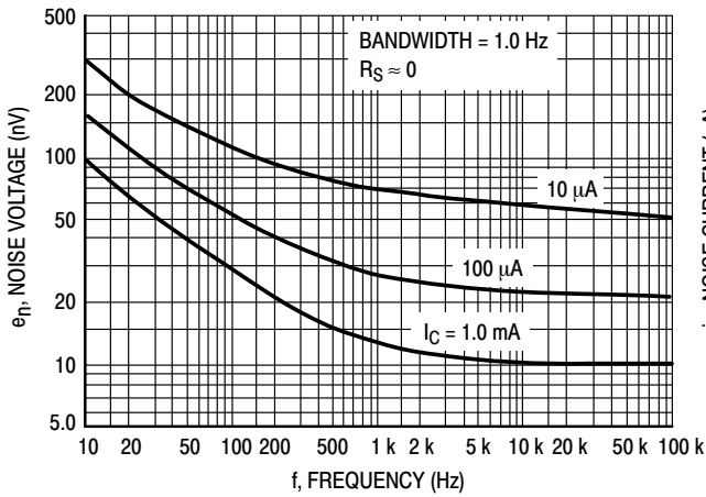
Figure 2. Noise Voltage
