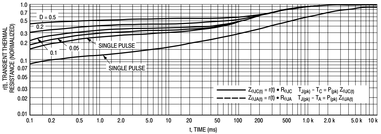
Figure 12. Thermal Response
