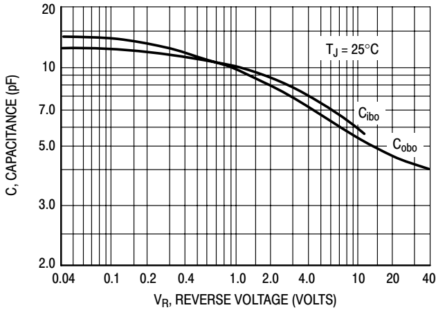
Figure 6. Capacitance
