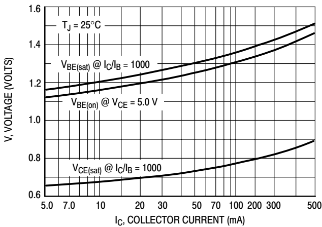
Figure 10. "On" Voltages
