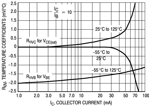
Figure 8. Temperature Coefficients NPN 2N6515, 2N6517
