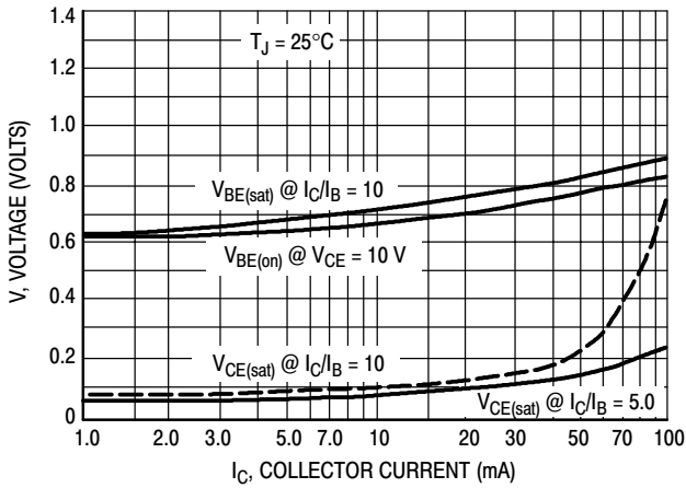
Figure 6. "On" Voltages NPN 2N6515, 2N6517
