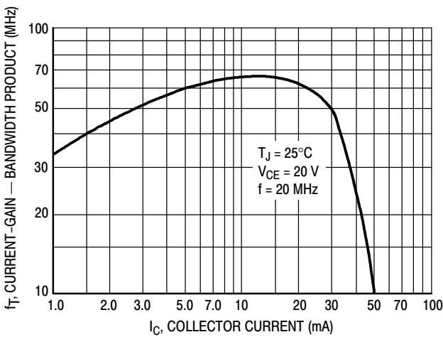
Figure 4. Current-Gain - Bandwidth Product NPN 2N6515, 2N6517
