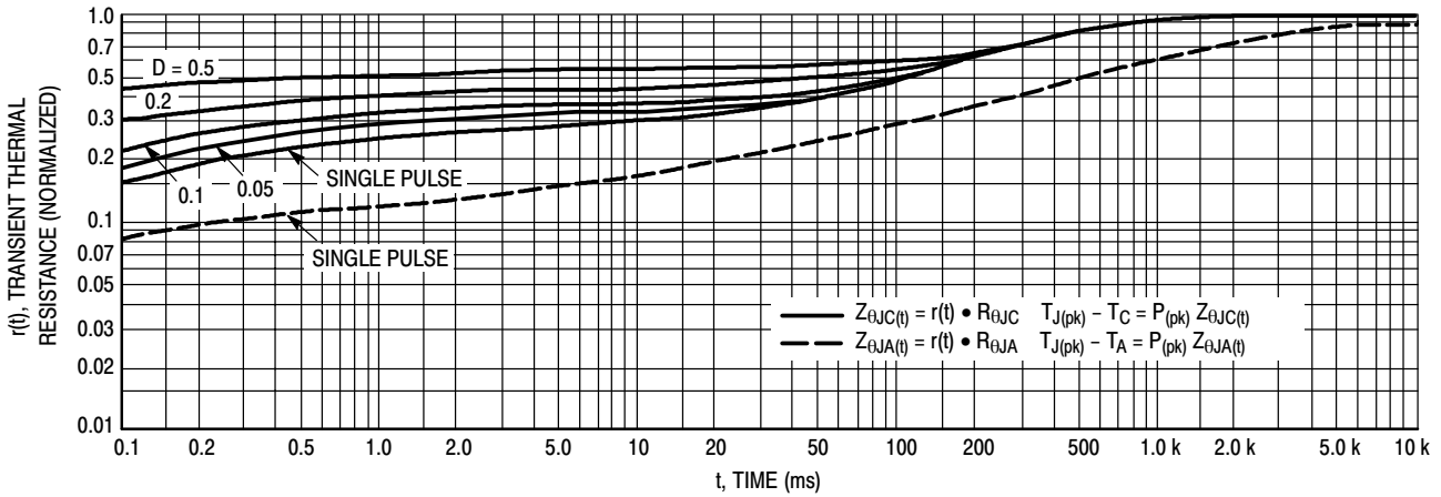
Figure 17. Thermal Response
