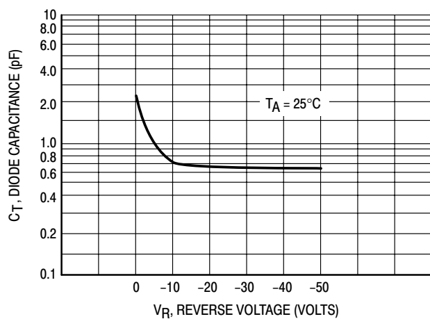
Figure 3. Diode Capacitance
