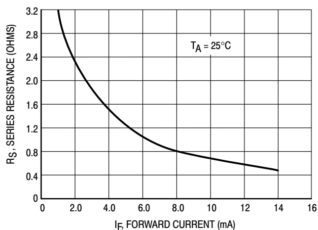
Figure 1. Series Resistance
