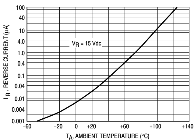
Figure 4. Leakage Current
