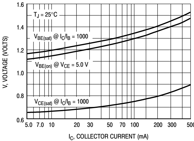
Figure 4. "ON" Voltages
