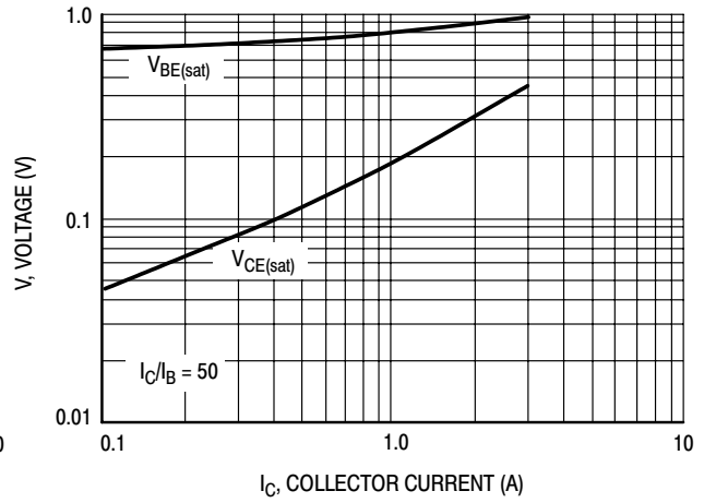
Figure 6. "On" Voltages
