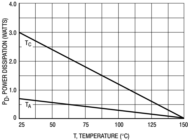
Figure 11. Power Derating
