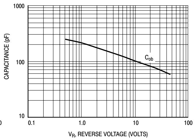
Figure 8. Output Capacitance
