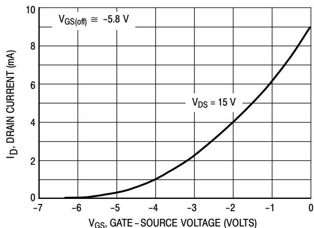
Figure 7. Common Source Transfer Characteristics
