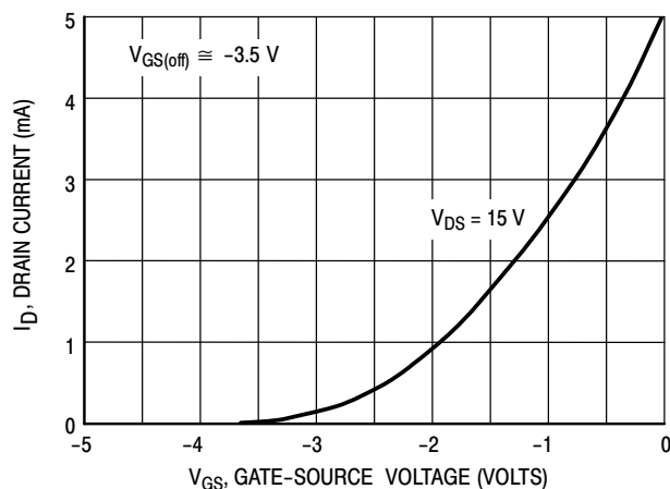
Figure 5. Common Source Transfer Characteristics
