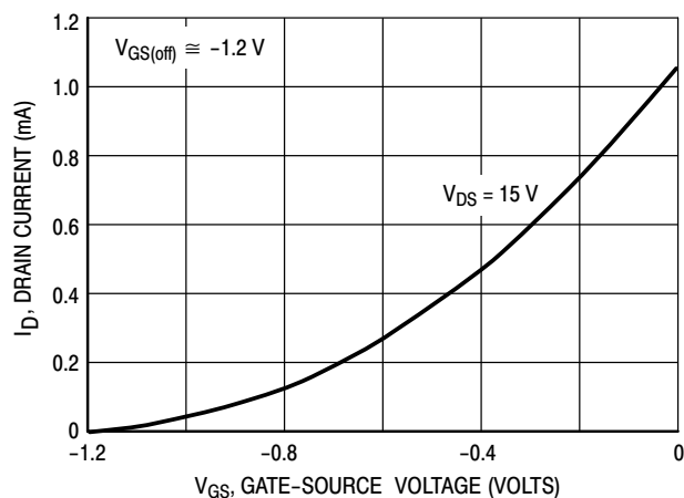
Figure 3. Common Source Transfer Characteristics
