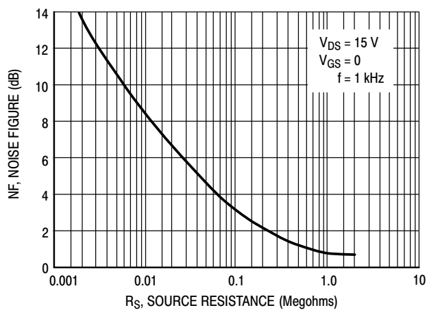
Figure 1. Noise Figure versus Source Resistance
