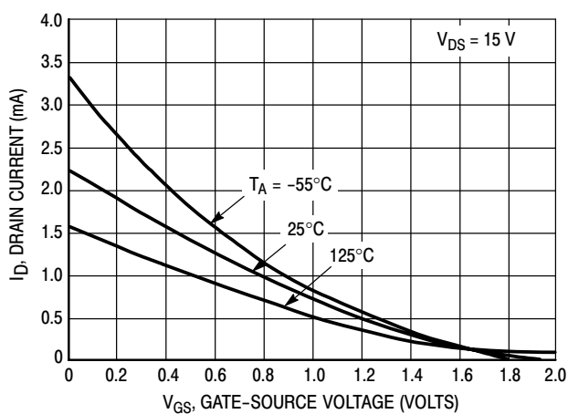
Figure 1. V_{GS(off)} = 2.0 Volts
