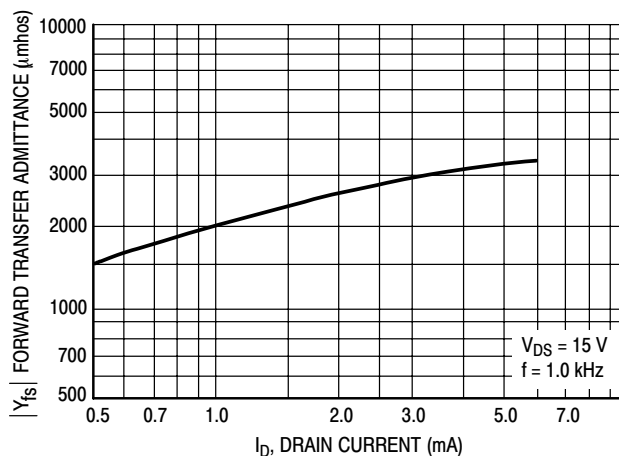
Figure 5. V_{GS(off)} = 4.0 Volts
