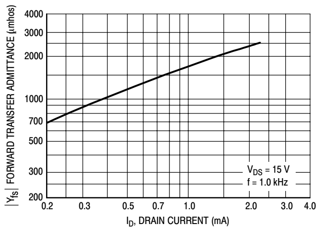
Figure 4. V_{GS(off)} = 2.0 Volts
