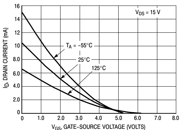
Figure 3. V_{GS(off)} = 5.0 Volts
