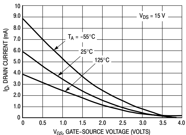
Figure 2. V_{GS(off)} = 4.0 Volts
