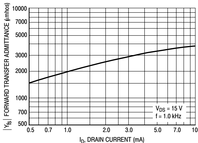
Figure 6. V_{GS(off)} = 5.0 Volts
