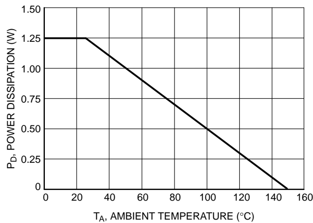
Figure 7. Power Derating
