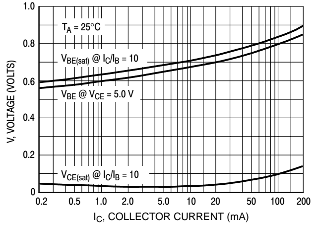
Figure 8. "On" Voltage
