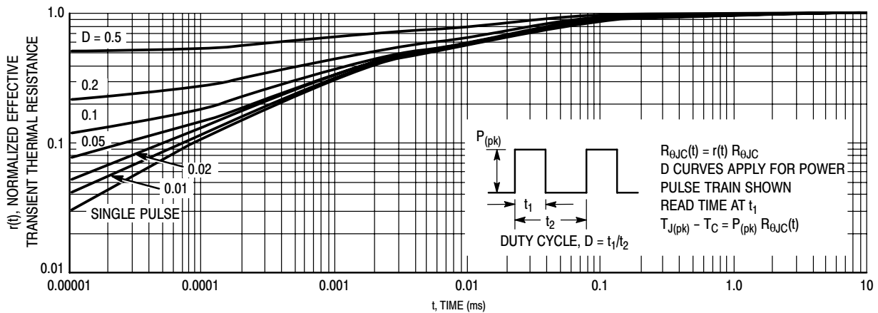
Figure 13. Thermal Response
