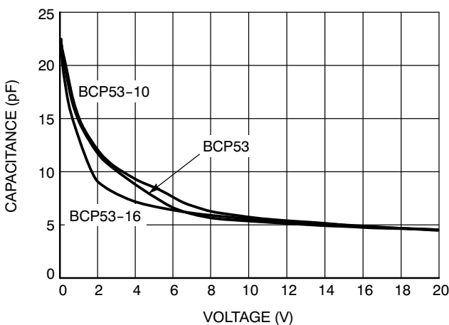
Figure 11. Output Capacitance
