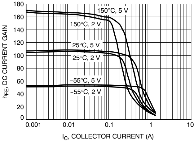
Figure 3. DC Current Gain vs. Collector Current (BCP53-10)
