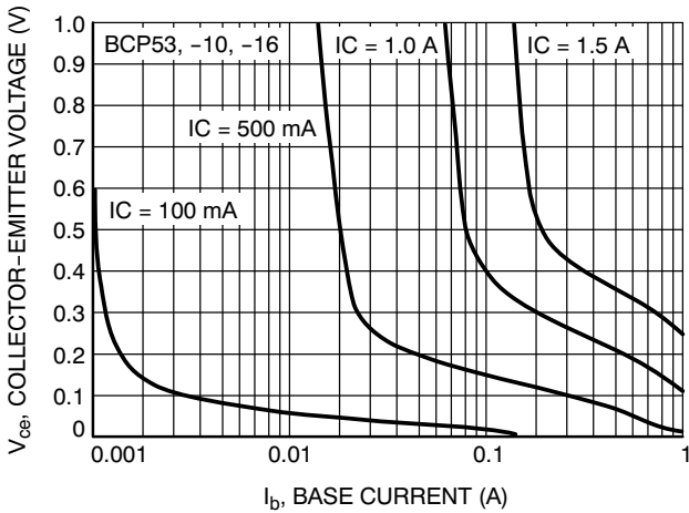
Figure 9. BCP53, -10, -16 Saturation Region
