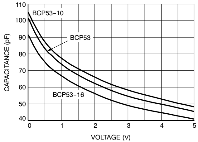
Figure 10. Input Capacitance
