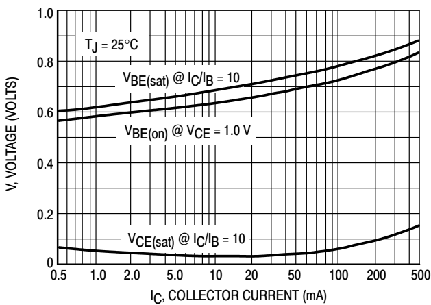
Figure 4. "On" Voltages
