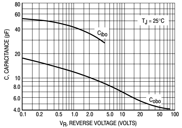
Figure 3. Capacitance
